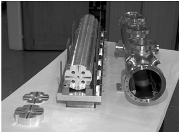
Figure 3: The structure being assembled.
