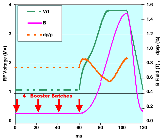
Figure 2: RF voltage programme and magnet cycle of the driver and evolution of momentum spread.
