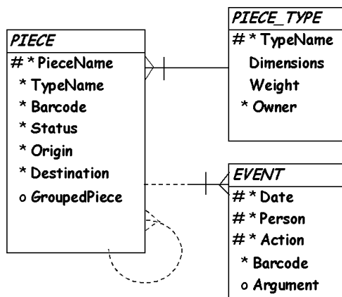
Figure 3: ERD for LEP traceability data.
