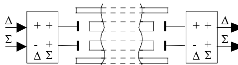
Figure 1: Schematic test set-up; port1=left; port2=right.
