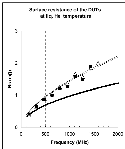
Figure 3: Surface resistance measured at 2K for a sample with smooth ( \Delta ) and another with ribbed ( \blacksquare ) surface. Solid line: RRR=90 from \rho(300\text{K})=2.15 \cdot 10^{-8} \Omega\text{m} , classical. Long dashed: RRR=90, \rho(300\text{K})=2.15 \cdot 10^{-8} \Omega\text{m} , anomalous. Dashed line: RRR=80, \rho(300\text{K})=1.7 \cdot 10^{-8} \Omega\text{m} , anomalous.
