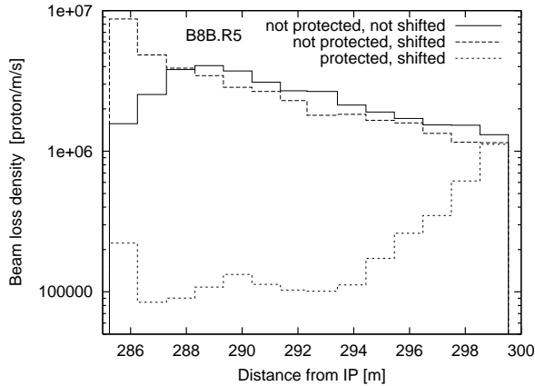
Figure 5: The beam loss density in the dipole B8B of the dispersion suppressor of IR5 at the nominal luminosity. Solid histogram: no collimators in the straight section and perfect alignment of B8B. Dashed histogram: same but with transverse displacement ( \Delta x=4\text{mm} , \Delta y=4\text{mm} ) of B8B. Dotted histogram: displaced B8B and collimator at Q5. IR1 data are very similar.
