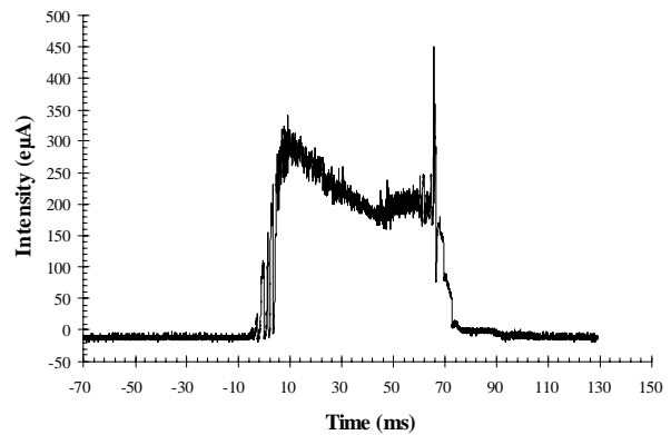
Figure 5: A \text{Xe}^{25+} beam pulse in afterglow mode.
