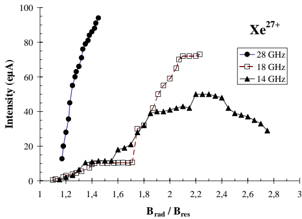
Figure 3: \text{Xe}^{27+} currents obtained by operating SERSE at different frequencies versus increasing radial field (20 kV extraction voltage).
