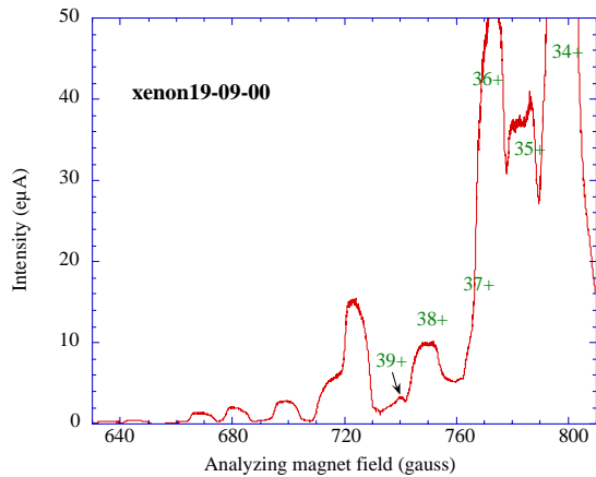
Figure 4: High charge states spectrum (power=4 kW).
