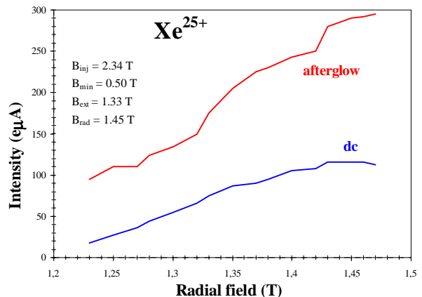
Figure 6: Comparison of \text{Xe}^{25+} currents in dc and afterglow mode versus the radial confining field.
