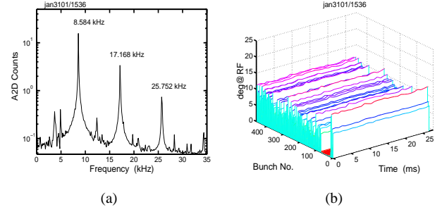
Figure 4: LFS data when the 180 Hz beam relaxation oscillation of Fig. 1 is damped by tuning the temperatures of the RF cavities at 121.39 mA, 2.5 GeV: (a) beam signal spectrum, (b) its time domain 400-bunch synchrotron oscillation amplitudes.
