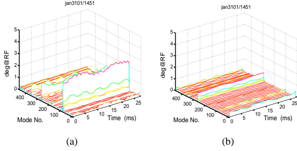
Figure 2: LFS data when the 180 Hz relaxation oscillation of Fig. 1 is generated: (a) time evolution of the quadrupole CBMI's, (b) time evolution of the dipole CBMI's.
