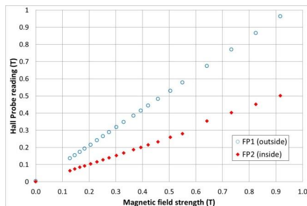
Figure 6: Field penetration measurements with Sample 2 ( \sim 1 \mu\text{m} thick Nb film on copper tube).
