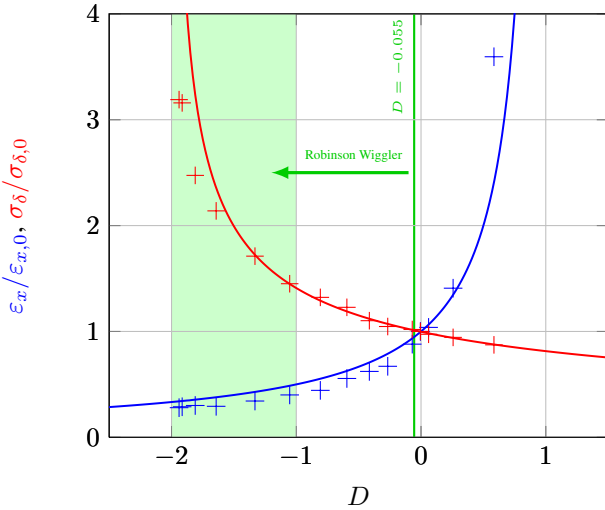
Figure 2: Effect of changing the damping partition D on energy spread \sigma_\delta and horizontal emittance \epsilon_x .
