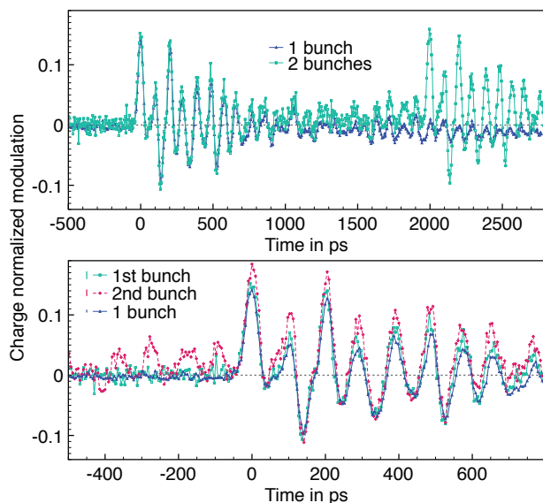
Figure 3: Top: Two EOS scans over a time range of 3 ns. One for a pure single bunch and one for a 2-bunch fill. The EOS-signal is normalized to the charge inside the first bunches. Bottom: Zoom into the region around the first peak for which in addition the signal of the second bunch has been displaced by -2 ns and has been normalized with the charge inside the second bunch.
