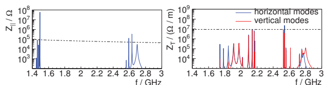
Figure 1: Longitudinal (left) and transverse (right) impedance of the JLab HC cavity compared to present BESSY II feedback performance (dashed line).
