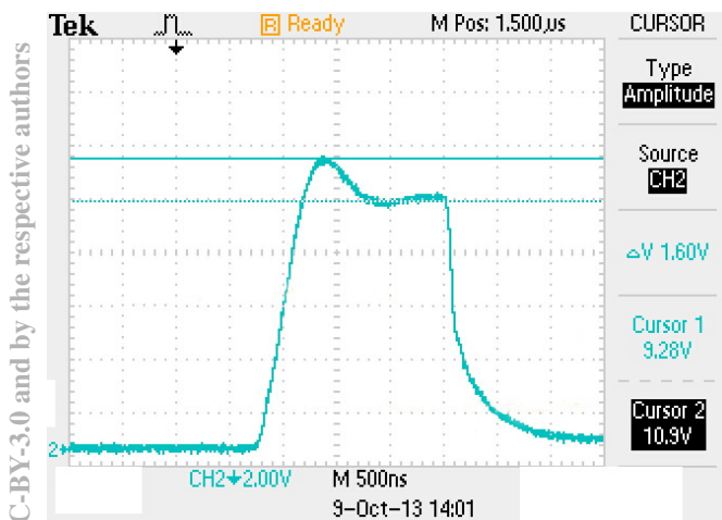
Figure 2: 280 kV, 185 A pulse from 29 Yale Marx modules into 1500 Ohm load, with intentional initial overshoot to reduce risetime. Ch2 (Blue): Current, 40A/div.
