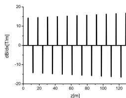
Figure 3: Quadrupole strength along the undulator.
