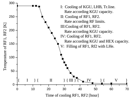
Figure 2. Cooling down of the RF separator superconducting cavities by CVS.
