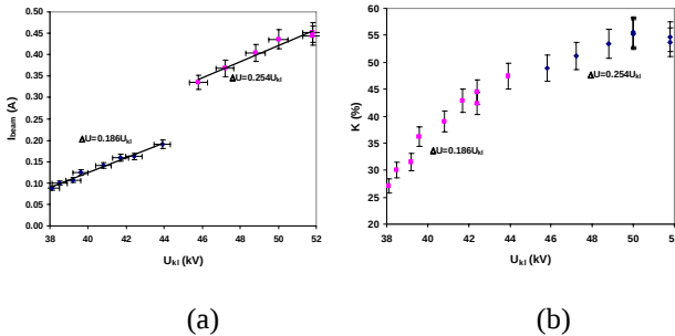
Figure 4: Dependence on high voltage pulse amplitude of (a) pulsed beam current and (b) capture efficiency.
