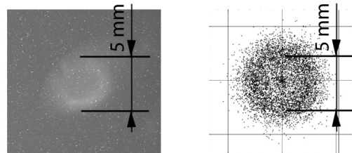
Figure 9: Registered by CCD camera and calculated beam images at 15 A.
