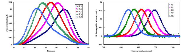
Fig. 2. Scan results presented by wire overheating temperatures (left) and recovered profiles from separate wires (right).
