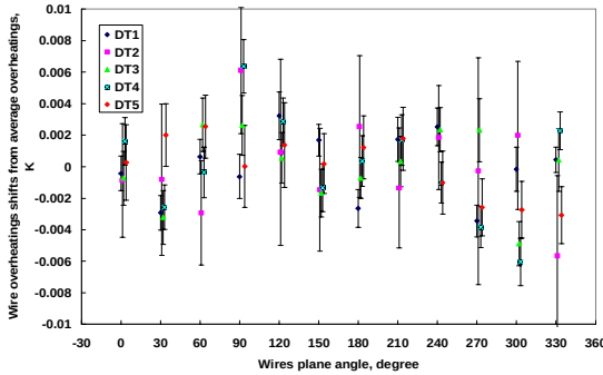
Fig. 4. Wire overheating dependence on the wires' plane rotation angle.
