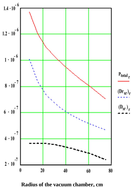
Figure 2: Averaged distributions of pressures in the vacuum chamber of the MCC-30/15 cyclotron ( P_{total} is the gas mixture pressure; Dr_{sr} is the partial pressure of hydrogen and D_{sr} is the partial pressure of nitrogen).
