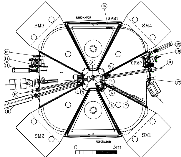
Figure 4: Layout of the SSC.
