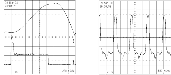
Figure 10: Magnetic guide field (ray A) and signal of deuteron beam from DCCT in the U1.5 (ray B) (left). Deuteron bunch at 1.18 T and RF 2.212 MHz (right).
