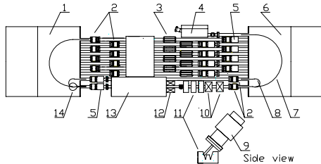
Figure 1: RTM schematic.
