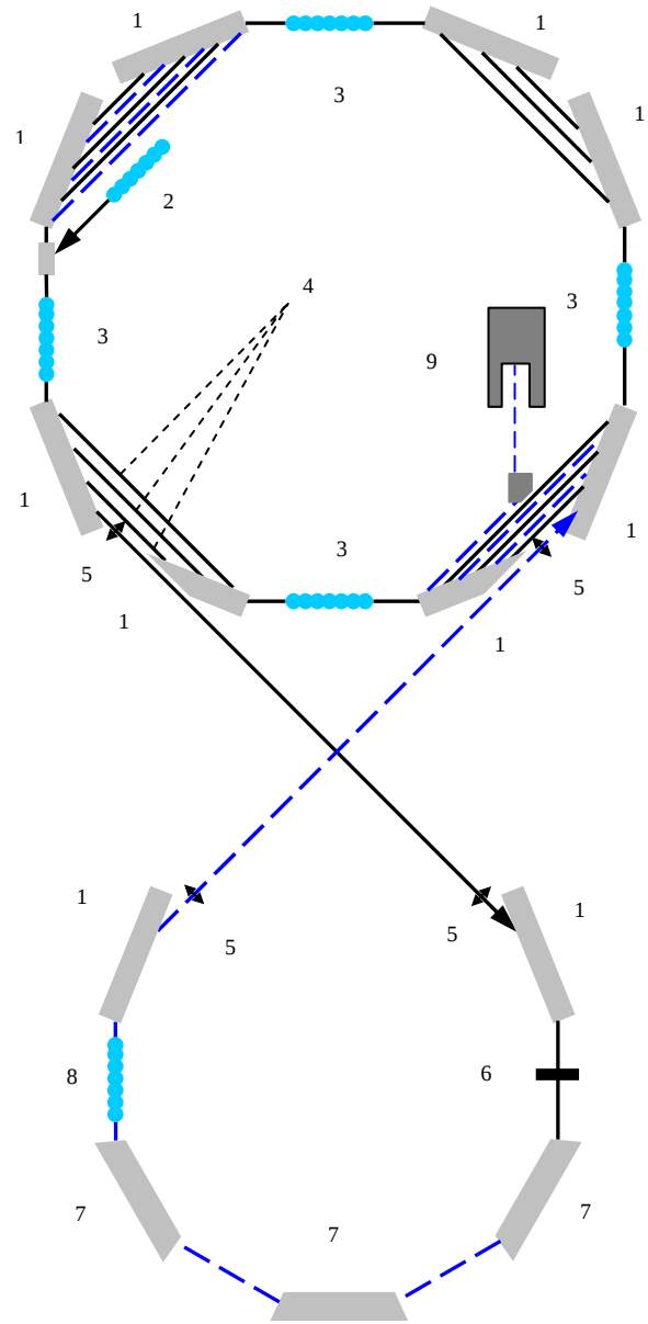
Fig. 1. Forth order politron with beam energy recovery system. 1 – magnet doublet, 2 – injector, 3 – superconducting linac, 4 – electron trajectories (dashed lines correspond to recovery beam), 5 – magnetic lens, 6 – target, 7 – achromatic magnet bending system, 8 – energy and spectrum correction linac, 9 – low energy electron beam absorber.
