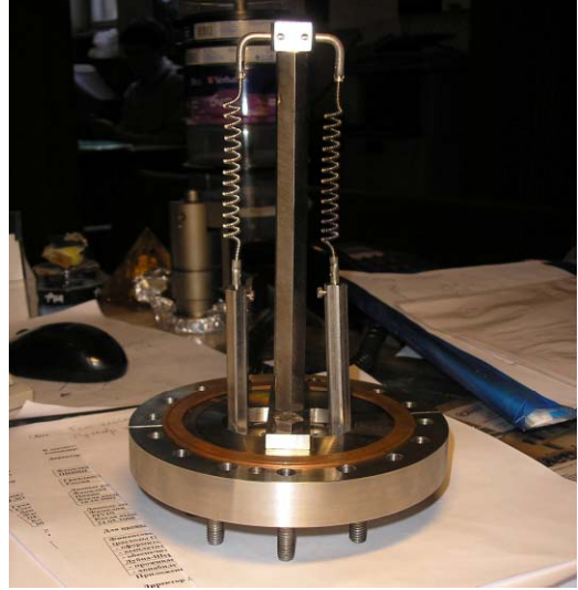
Figure 4: The evaporated getter pump
