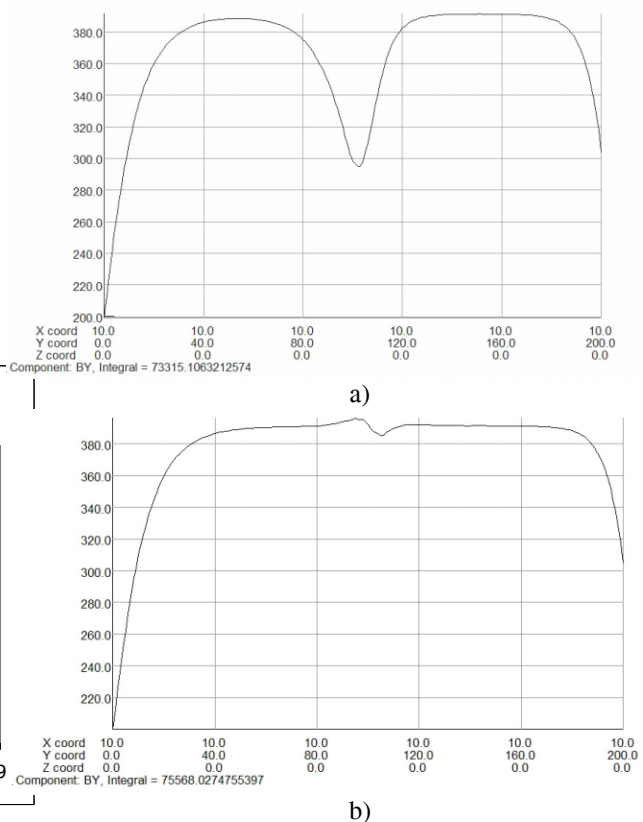
Figure 5: The inhomogeneities of magnetic field
