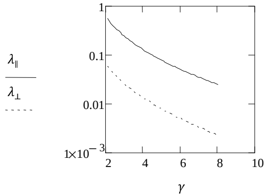
Fig.2. Dependence of cooling rates \lambda_{\parallel} and \lambda_{\perp} (in logarithmic scale) versus the relativistic parameter \gamma for \epsilon = 10^{-6} m \cdot rad and \sigma_p = \frac{\Delta p}{p} = 10^{-4} .
