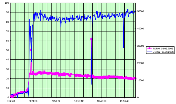
Fig. 5. The lifetime(blue) and the losses rate(red) as function of the time at ramping and pending circulation at the energy 2.5 GeV. Growth of losses rate fit with decay of the lifetime.
