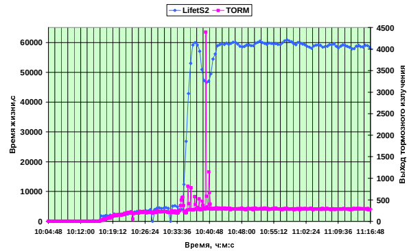
Fig. 7 The lifetime and the losses rate during changing of the beam orbit.
