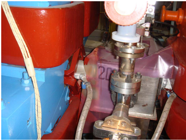
Fig. 3 BLM placed on the box of pumping and diagnostics inside the ring.
