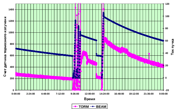
Fig. 6 The beam current (black) and the losses rate (red) in 24 of hours. Growth of losses rate conform to increasing of the pressure into the vacuum chamber.
