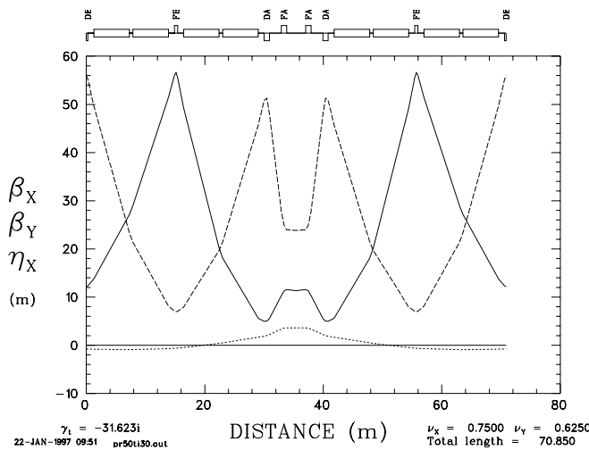
Fig: 3 Lattice functions and dispersion for an arc cell.
