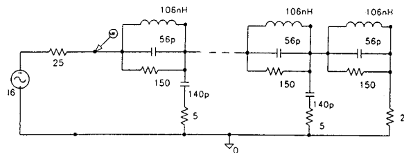
Figure 3: Equivalent circuit of injection kicker. Only 3 of the 14 dielectric capacitors in a full-length kicker are shown.
