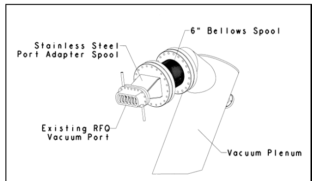
Fig. 2 RFQ Vacuum Port Adaptor Spool & Bellows Assembly
