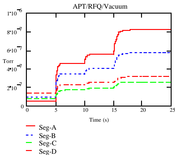
Fig. 3 Analysis Results of Simulation of Loss of Pumps in Segment A.
