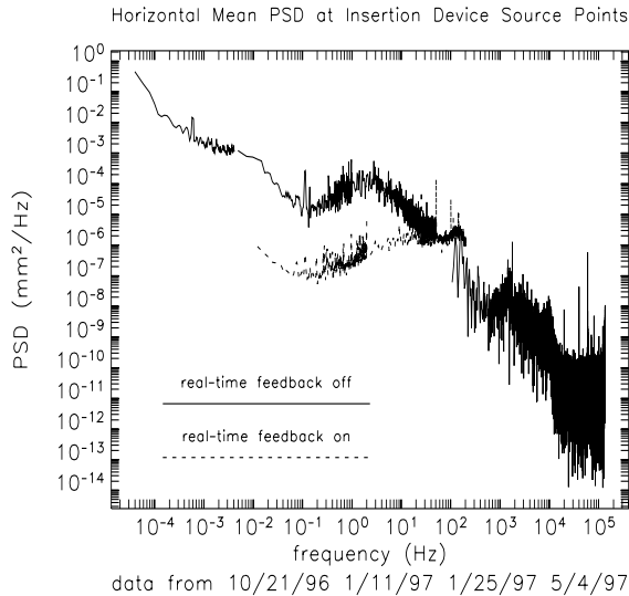
Figure 4: Horizontal spectrum with and without feedback.
