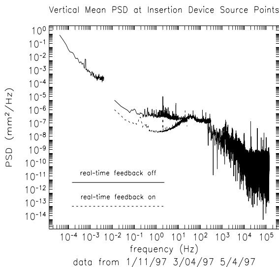
Figure 5: Vertical spectrum with and without feedback.
