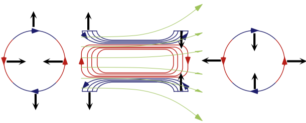
Figure 4: Forces acting on a quadrupole magnet due only to the B_z component of the solenoid field
