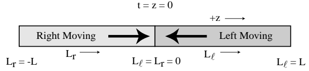
Figure 1: Configuration and coordinates for the calculation. L_r and L_\ell are right-handed coordinates that move with the beams. The figure is drawn at the start of the interaction.
