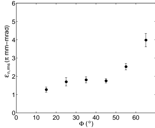
Figure 4: \epsilon_{n,rms} versus \phi
