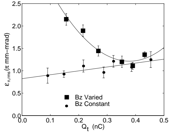
Figure 3: \epsilon_{n,rms} versus Q_t
