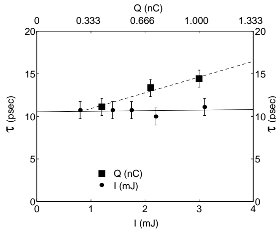
Figure 5: \tau_{95\%} versus I_{green} with Q_t constant. \tau_{95\%} versus Q_t with I_{green} constant.
