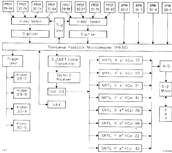
Fig. 2. Detailed components of the transverse feedback system.
