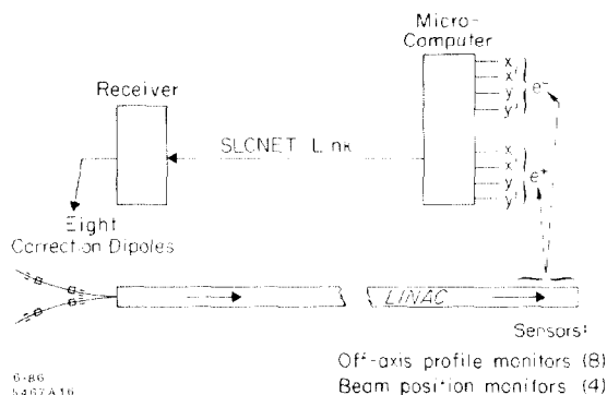
Fig. 1. Transverse feedback system for the linac.
