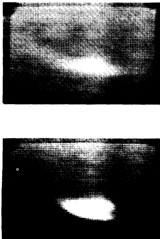
Fig. 5. Photographs of beam spots at 1.8 \times 10^{10} e^- at 43 GeV. The upper photograph shows a horizontal tail on the beam core, and the lower photograph shows a vertical tail, both induced by wakefields and chromatic-dispersive effects. The fiducial holes have separations of 3 mm (h) by 1 mm (v).
