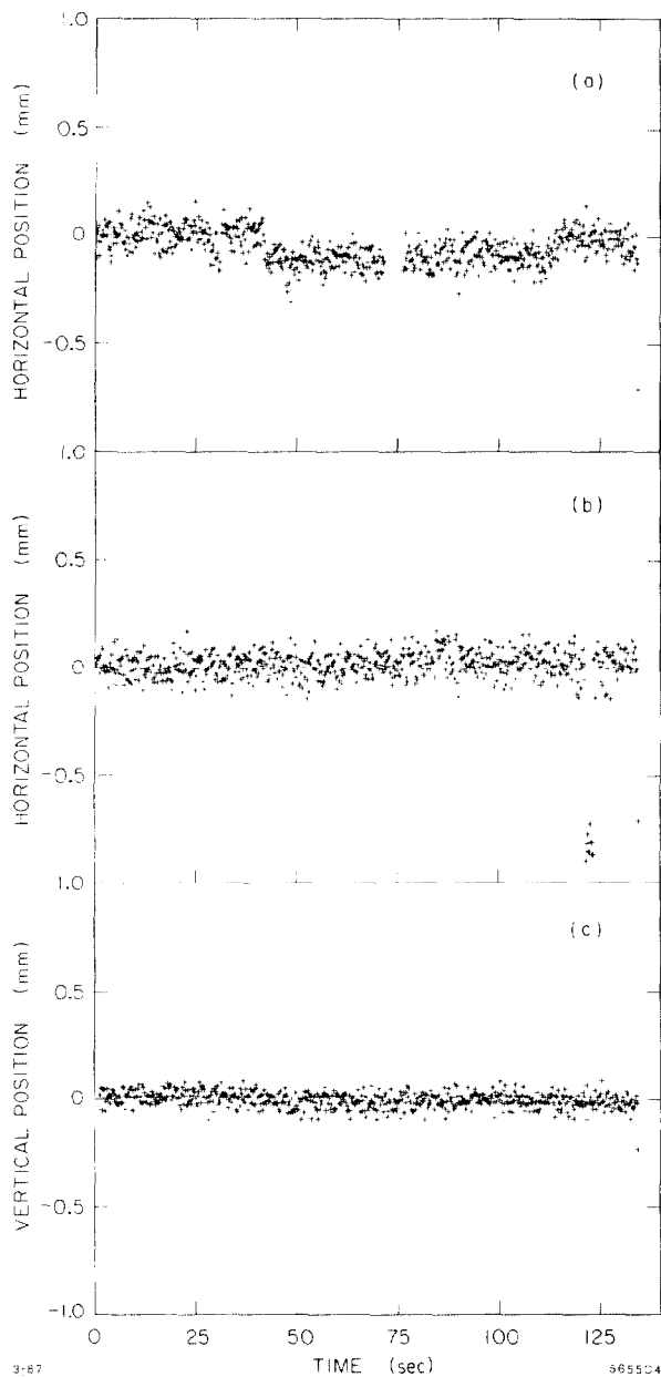
Fig. 4. Measured position jitter at the end of the linac at 8 \times 10^9 e^- , 47 GeV, and 5 pps: (a) shows a horizontal position shift correctable by feedback, (b) and (c) show more typical open loop horizontal and vertical jitter plots. The horizontal jitter is 120 \mu\text{m} rms and the vertical 30 \mu\text{m} .
