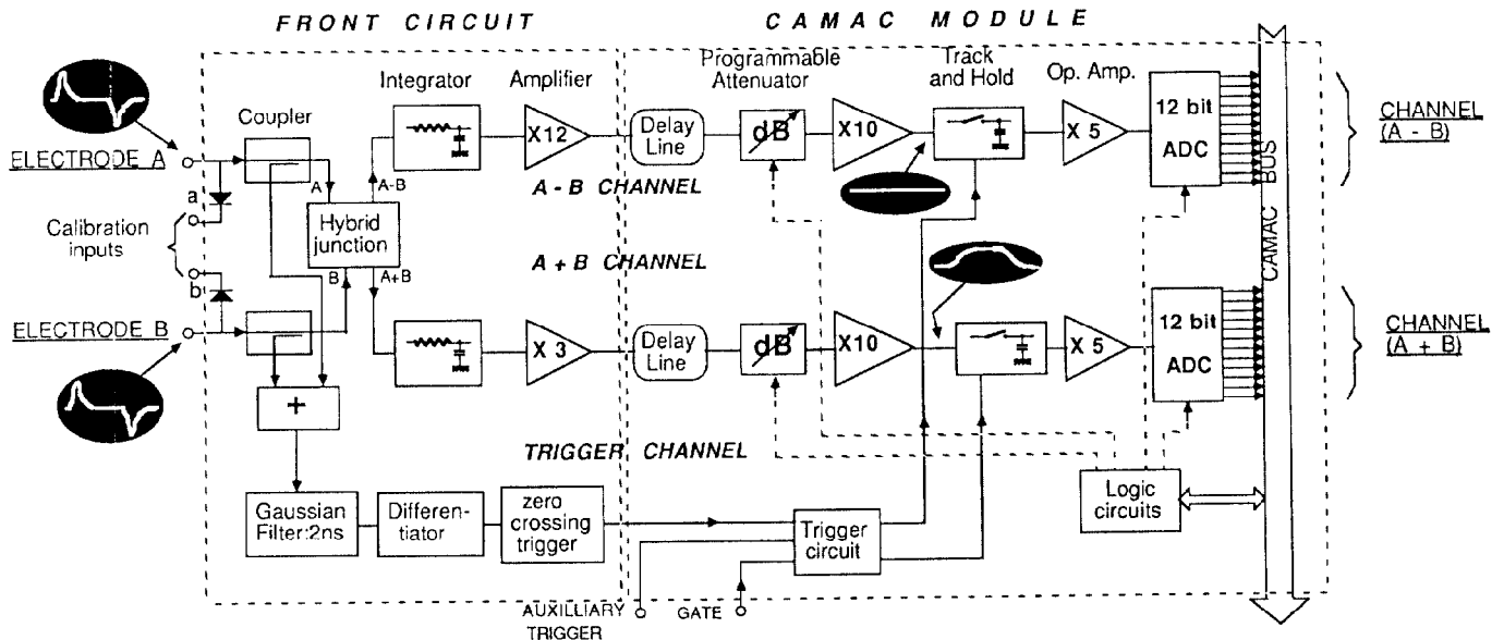
Figure 5: Block diagram of the processing electronics.
