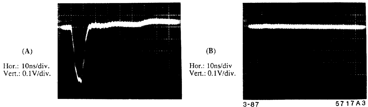
Figure 4: Directivity of an electrode after integration. A short impulse (400ps), injected in a coaxial rod inside the monitor, simulates the beam. The rod and the monitor form a 50\Omega transmission line matched at the end.
