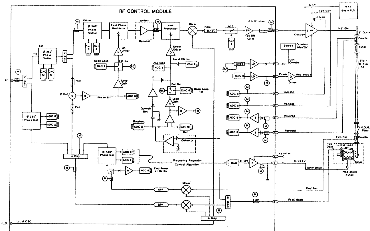
RF CONTROL SYSTEM
