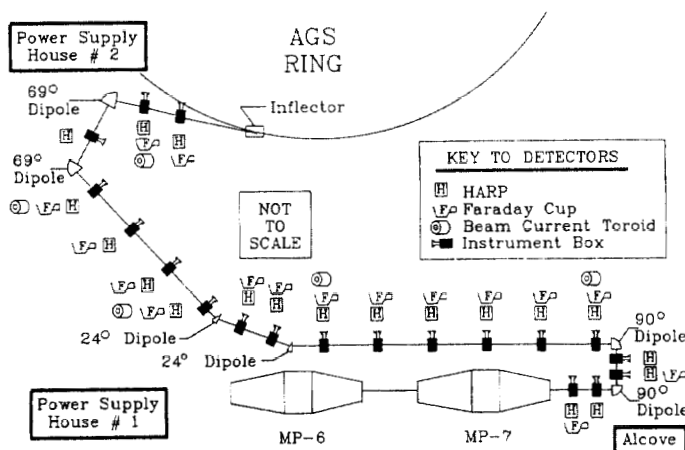
Figure 2. Locations of beam instrumentation in HITL.
