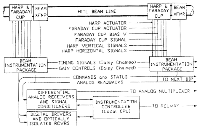
Figure 1. Beam instrumentation signal flow in HITL.
