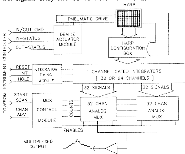
Figure 4. Block diagram of the HARP electronics.
