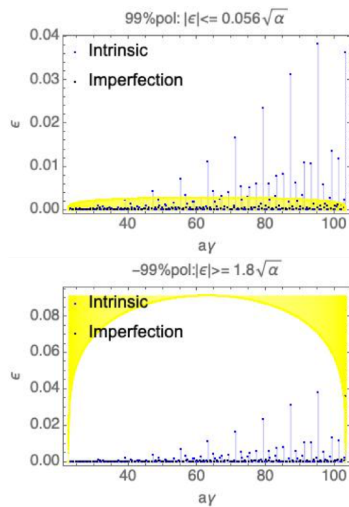
Figure 3: Spin resonance spectral of CEPC booster, in yellow region 99% initial polarization is maintained after resonance cross. The upper and lower plots show the fast crossing and adiabatic crossing scenarios, respectively.
