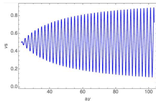
Figure 4: Evolution of the closed orbit spin tune in CEPC booster with a non-ramping solenoid snake.
