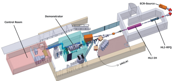
Figure 2: Demonstrator environment at GSI.
