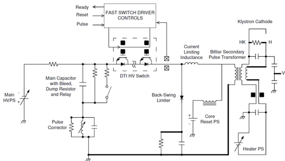
Figure 2. Simplified modulator schematic. Directly switching 35 kV on the primary simplifies the pulse transformer and improves the risetime compared to higher step-up ratio designs. Series IGBT switches have inherent redundancy such that several modules may fail before system performance is affected.
