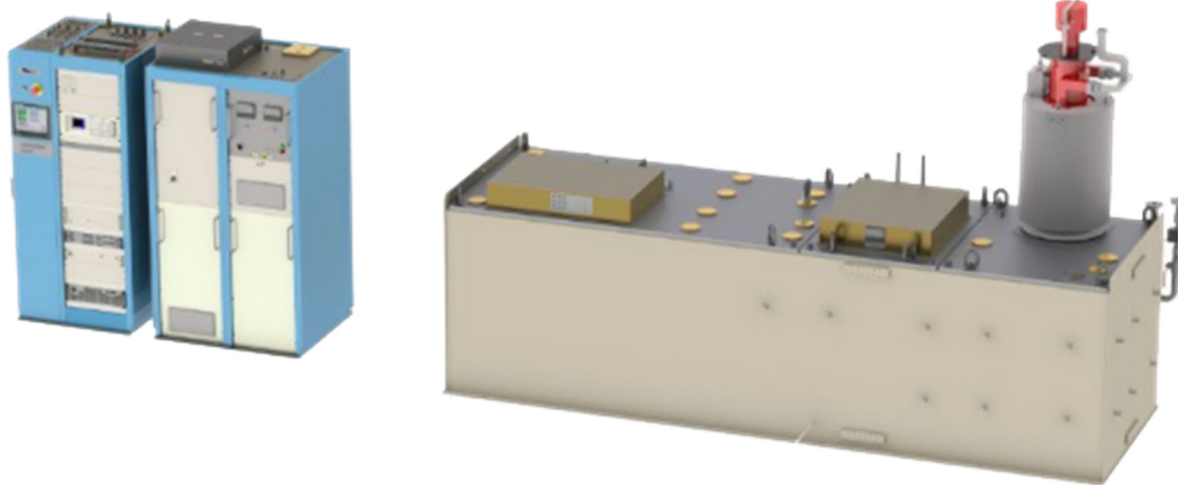
Figure 1: 250 MW Peak Power CLARA Klystron Modulator System. High voltage solid-state switching allows a simple and reliable modulator with extremely high pulse fidelity and stability. One rack houses low voltage circuitry and controls (left) while a double-wide rack houses DTI's standard high voltage power supply and step-up AC transformer (center), allowing standard US 480 VAC input to the HVPS from 380 VAC British power.
