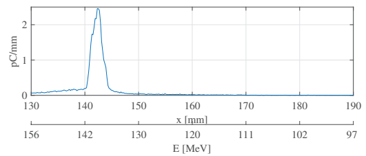
Figure 7: Particle distribution after spectrometer.
