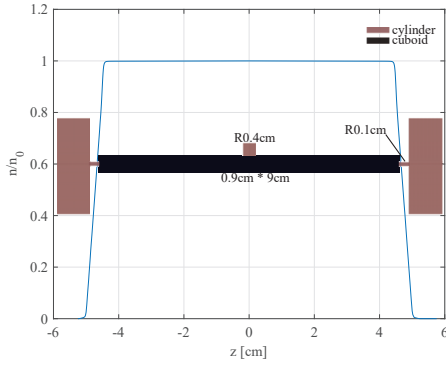
Figure 4: Schematic of the plasma cell and the on-axis density profile along the cell.
