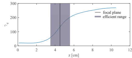
Figure 6: Energy gain along the plasma cell with a density 2 \times 10^{17}/\text{cm}^3 , the efficient acceleration range is within one Rayleigh length of the laser focal plane.
