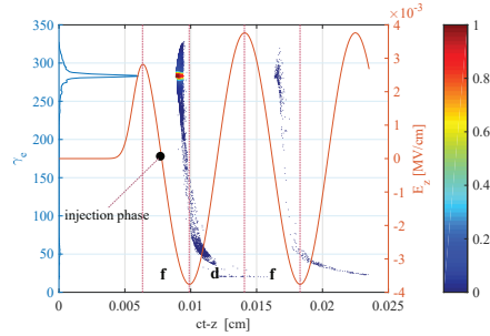
Figure 5: The electron distribution at the plasma ( 2 \times 10^{17}/\text{cm}^3 ) exit. The longitudinal electric field is from 0.6 cm of plasma exit, is only used to show the optimal injection phase (near the solid circle) and phase slip process.
