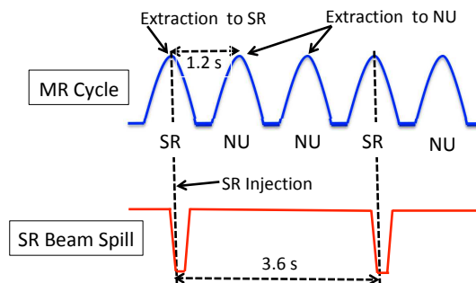
Figure 1: Stretcher ring scheme for the slow extraction.
