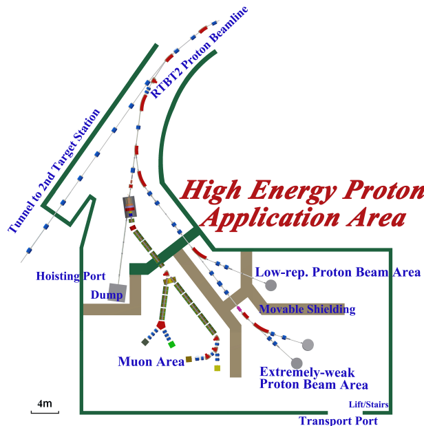
Figure 1: Schematic layout of the high-energy proton application area including the EMuS beamlines at the CSNS campus.
