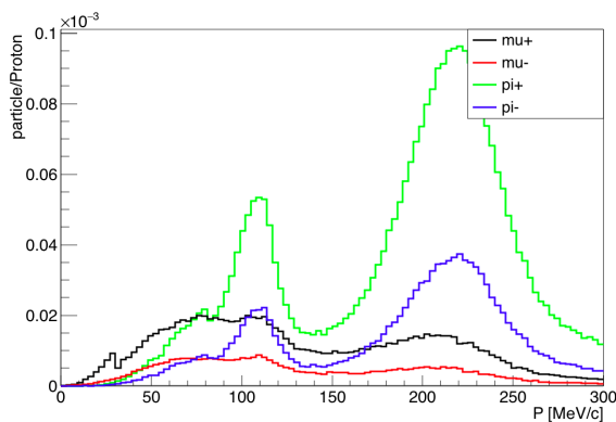
Figure 5: Momentum distributions of the muons and pions at the end of the capture solenoid. The solenoid is optimized to capture pions with momenta of 230 MeV/c.
