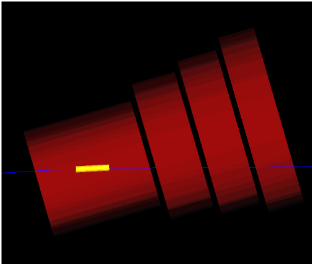
Figure 2: Schematic layout of the target station. The target (yellow) sits at the center of the first coil with an angle of 16^\circ and the protons (blue line) hit the target and get through the target station to the downstream beam dump.
