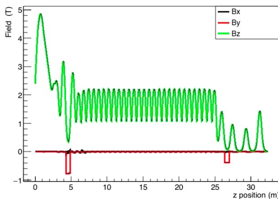
Figure 6: Magnetic field along the decay muon beamline.
