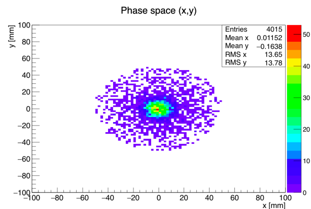
Figure 4: Beam spot at the sample area after collimating the beam by a size of 50 mm in radius.
