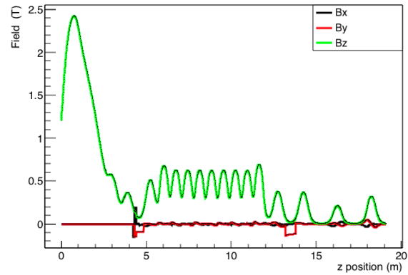
Figure 3: Magnetic field along the surface muon beamline. The green line is B_z field representing the solenoids, and the red line is B_y field indicating the positions of the bending magnets.
