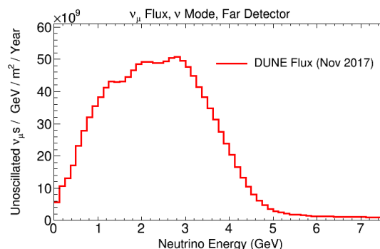
Figure 5: Neutrino mode flux of muon neutrinos as a function of neutrino energy for the recently optimized beam design.
