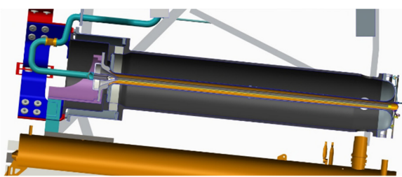
Figure 4: The optimized LBNF target mounted into the first horn. The proton beam comes from the left. The helium supply line is shown in light blue.
