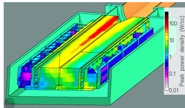
Figure 7: Shower energy deposition in first secondary collimator for a 12 minute beam lifetime.
