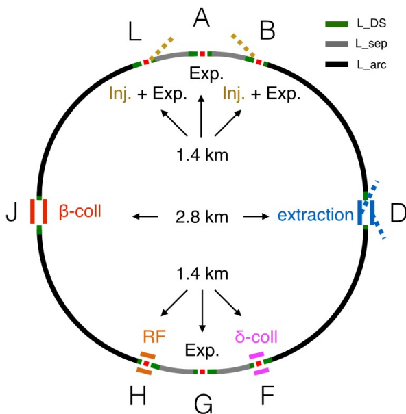
Figure 6: FCC-hh layout with 8 straights.
