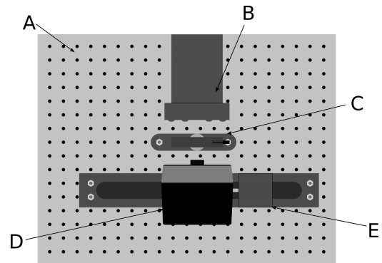
Figure 4: Schematic diagram of the CLARA Phase 1 proposed experimental apparatus: A - optical breadboard, B - quartz window, C - polyethylene polariser (rotatable), D - x-y translation stage, E - gentech-eo PE detector
