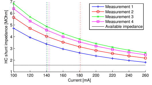
Figure 1: Required HC shunt impedance in MAX II to reach flat potential conditions simulated with Code 1. The vertical lines indicate the four measurement currents presented in Table 3.
