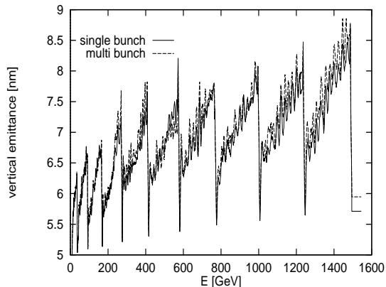
Figure 5: Emittance variation along the main linac.
