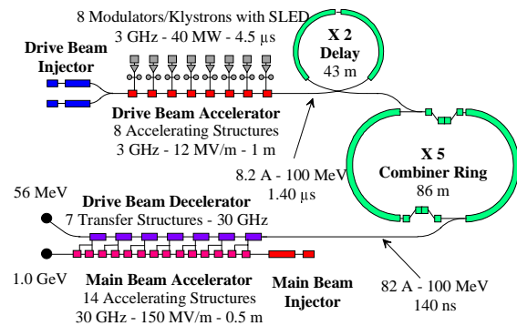
Figure 9: CTF3 schematic layout.
