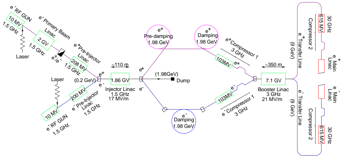
Figure 7: Layout of the injector complex of the main beams.
