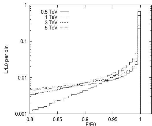
Figure 4: Luminosity distribution with energy.
