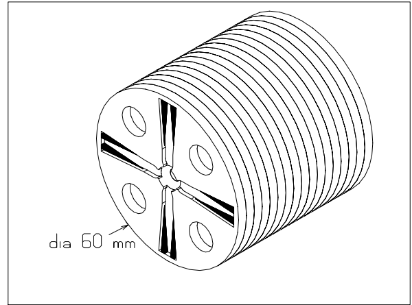
Figure 6: 30 GHz Tapered Damped Structure.
