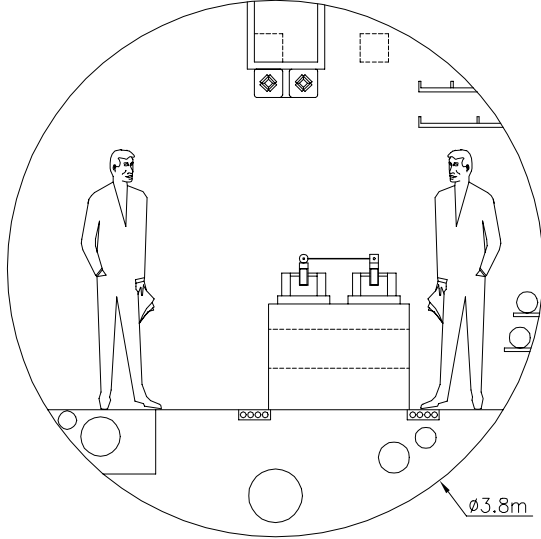
Figure 2: One main beam and drive beam module.
