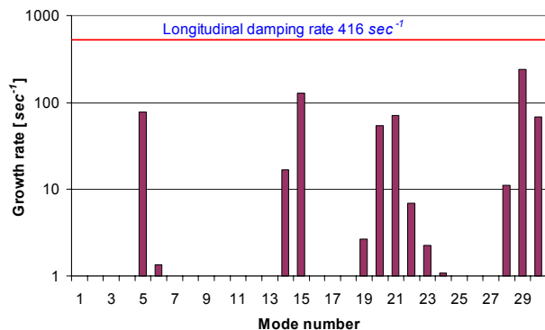
Figure 3: Growth rate of the LCB modes with the measured HOM's frequencies in one cavity and then assuming three identical cavities.
