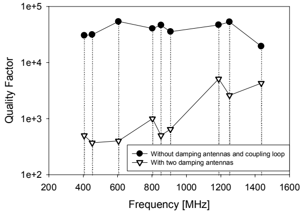
Figure.2: Measured Q-values of the longitudinal HOM's. Lower curve with 50Ω termination on the coupling loop.
