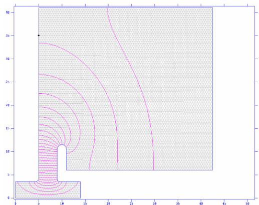
Figure 1: 100 MHz cavity profile with fundamental mode E-field lines.
