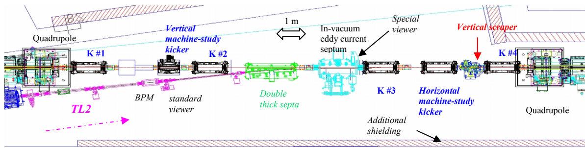
Figure 2: Injection straight section with pulsed magnets and diagnostics
