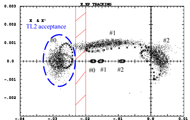
\square and * Ideal injected beam contour without any error in Booster-TL2 \cdot Simulated injected beam for tracking with conservative distribution + Bumped stored beam
