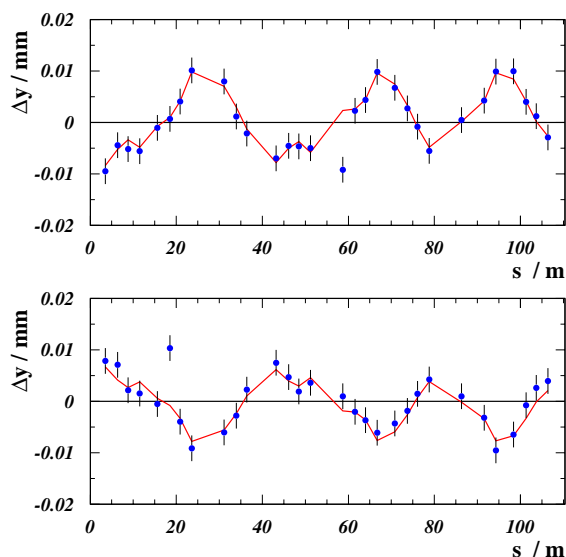
Figure 1: Difference in vertical closed orbit between measurements with and without scraper as a function of BPM position for a top scraper jaw position of 6mm (top plot) and a bottom scraper jaw position of 2.5mm (bottom plot). The opposite jaw is always out. The measurements were done for a total beam current of 120mA and 105mA, respectively, distributed equally over 30 bunches in one train. The solid line represents a fit of a MAD [3] model with scraper kick to the measured difference orbit.
