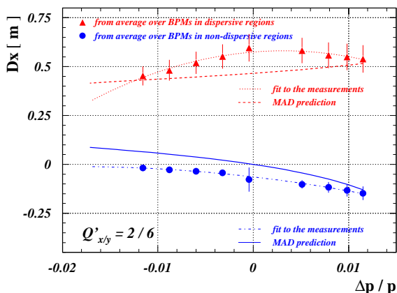
Figure 7: Horizontal dispersion as a function of momentum deviation obtained by changing the RF frequency for a horizontal chromaticity of 2 and a vertical chromaticity of 6. Measurements derived on the observation of the average horizontal closed orbit shift for beam position monitors in dispersive (triangles) and “non-dispersive” sections are shown as well as calculations with the MAD program are shown. The error bars reflect the scatter of the beam position measurements at different locations in the storage ring for a given momentum deviation.
