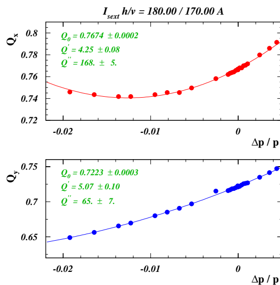
Figure 2: Measurement of the horizontal and vertical chromaticity. The points are measurements, the curves are fits to the measured data. The nonlinear shape clearly indicates the presence of higher order nonlinear terms like octupoles [2].
