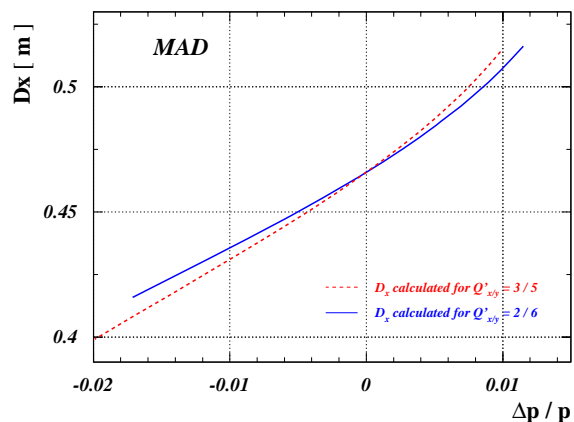
Figure 4: Horizontal dispersion as a function of momentum deviation as calculated by the MAD program for two different sets of horizontal and vertical chromaticities. The calculation was done for a beam position monitor located in a dispersive region in the storage ring. The nonlinearity of the dispersion in momentum deviation is clearly visible. There seems to be a divergence of the the dispersion for large positive \Delta p/p .
