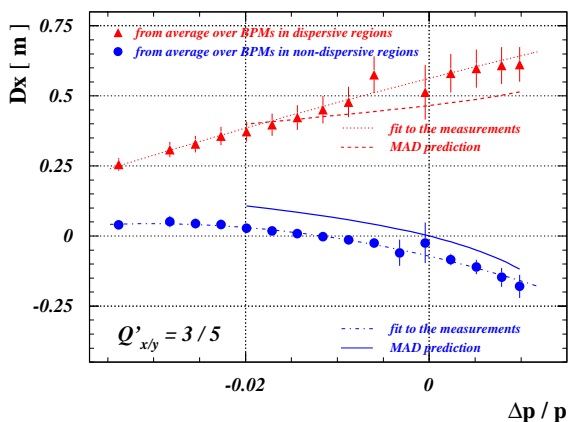
Figure 6: Horizontal dispersion as a function of momentum deviation obtained by changing the RF frequency for a horizontal chromaticity of 3 and a vertical chromaticity of 5. Measurements derived on the observation of the average horizontal closed orbit shift for beam position monitors in dispersive (triangles) and “non-dispersive” sections are shown as well as calculations with the MAD program are shown. The error bars reflect the scatter of the beam position measurements at different locations in the storage ring for a given momentum deviation.
