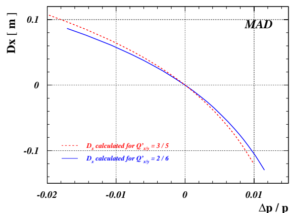
Figure 5: Horizontal dispersion as a function of momentum deviation as calculated by the MAD program for two different sets of horizontal and vertical chromaticities. The calculation was done for a beam position monitor located in a non-dispersive region in the storage ring. Again the divergence of the the dispersion for large positive \Delta p/p is pronounced.
