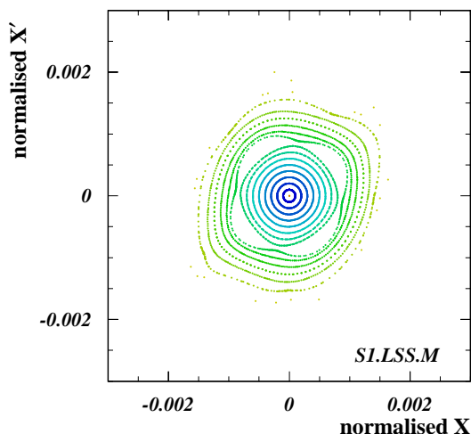
Figure 3: Horizontal phase space in the middle of the first long straight section generated with the MAD program [3] for the full nonlinear ANKA optics model.
