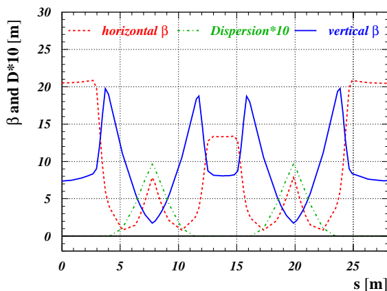
Figure 1: Horizontal and vertical \beta function and dispersion for \Delta p/p = 0 for one quarter of the ANKA storage ring. The dispersion has been scaled by a factor of 10 for better visibility.
