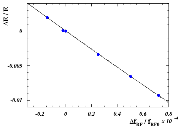
Figure 8: Relative energy change determined with resonant electron spin depolarisation [4] as a function of relative change in RF frequency. The dashed line is a straight line fit to the measurements, the solid curve a parabolic fit.
